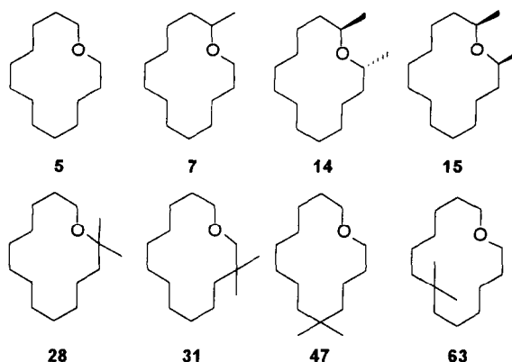
Figure 1. Macrocyclic ethers prepared in this study.
