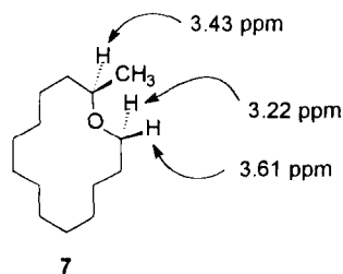
Figure 2. Selected ^1\text{H} NMR assignments of 7 from COSY and NOEDS experiments.
